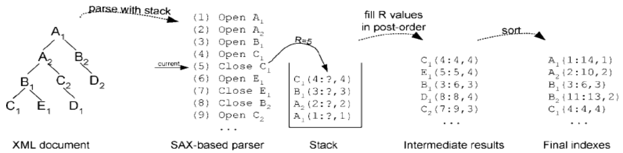
Figure 1 Index creation in index-filter technique
