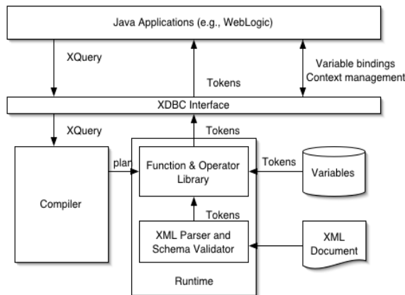
Figure 2 Overview of BEA
